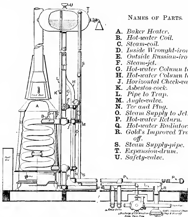
Fig. 3003. Sectional View of Heater and Pipe Connections.
